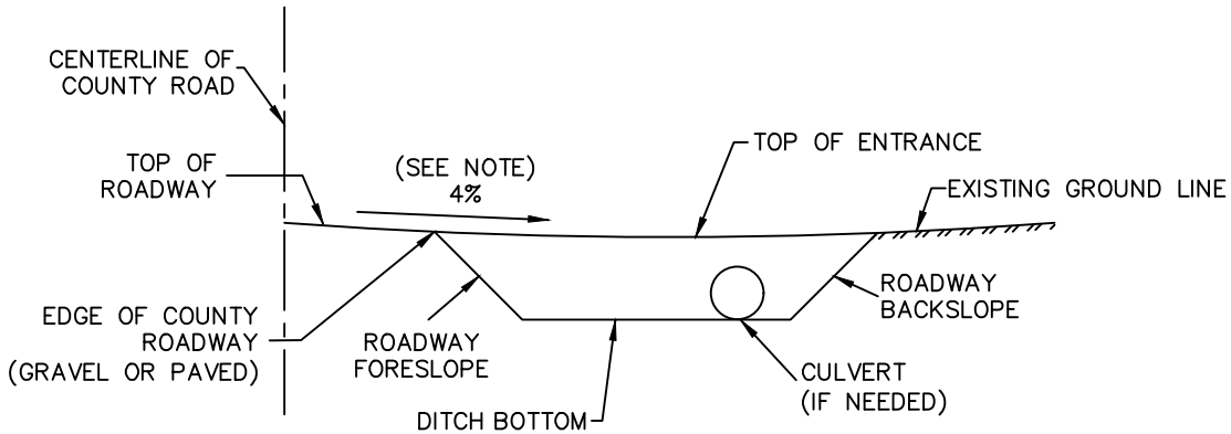
PROFILE VIEW
